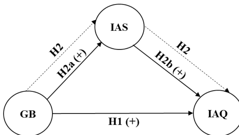
Figure 1: Research Framework
